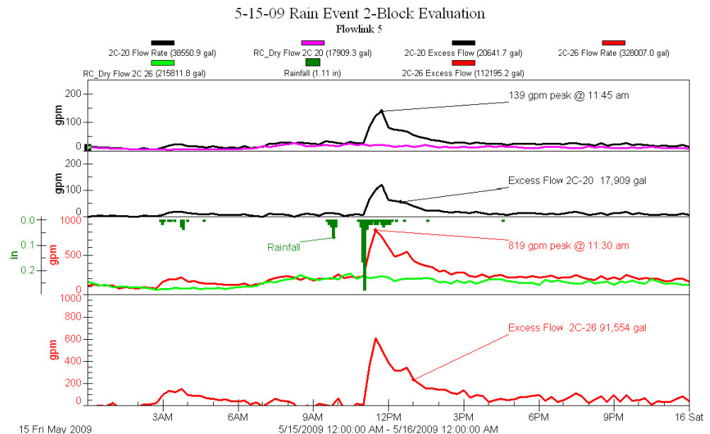
Figure 2: Rain event in Falls City, May 2009 Reference curve graphically depicted with Isco Flowlink® software
