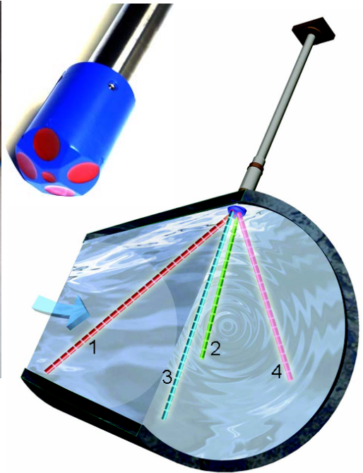
Figure 1: Hot Tap sensor installation and operation
