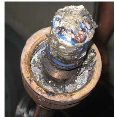
Figure 2: Sensor tip fouled w/ grease & sludge after nine months in service
