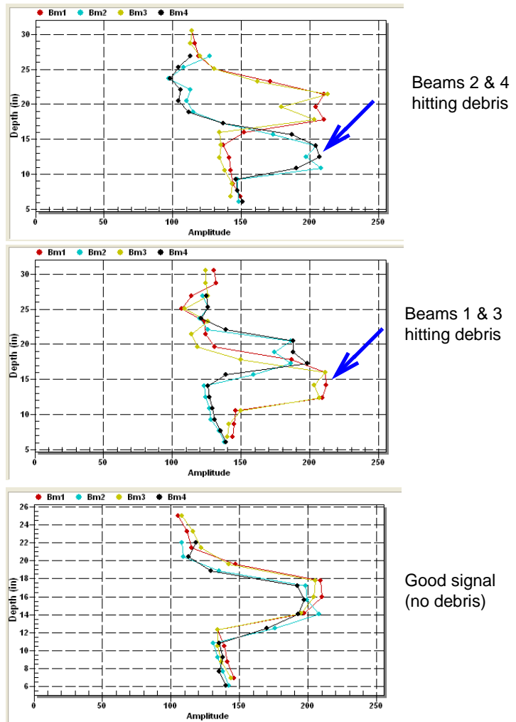
Figure 3: Velocity beam signals showing sediment build-up Challenge Met.
