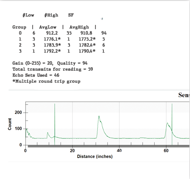
Diagnostic report shows the sensor is level and showing strong Doppler (left) and Ultrasonic (right) signal returns.
